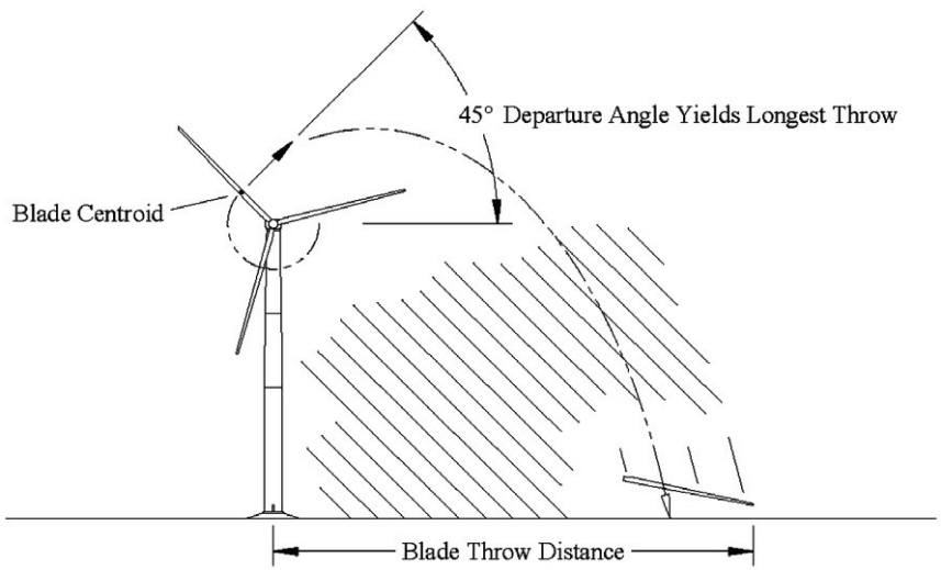
Inset B: Blade throw distance.
