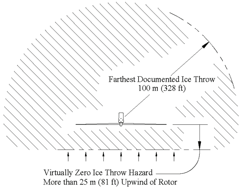
Inset C: Blade ice throw and blade fragment throw hazard zone.
